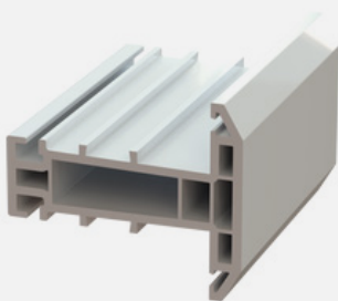
Sash Transom/Mullion
