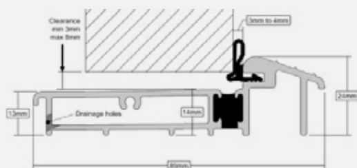
Proline AM5EX-78
