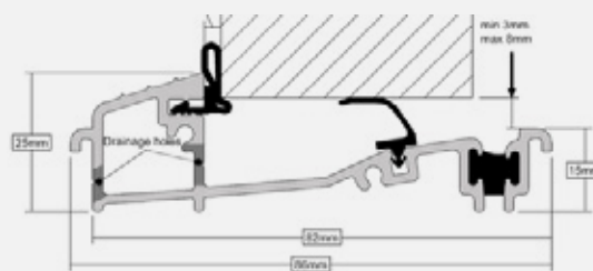
Proline AM3EX-78
